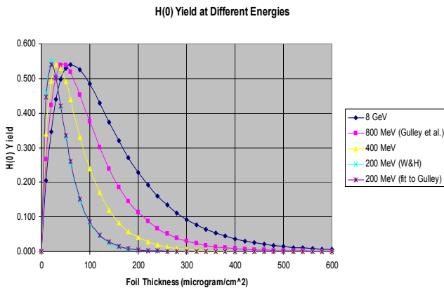
Figure 5: Unstripped H^0 vs. foil thickness at different energy of H^- ions.
