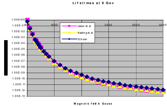
Figure 3: Prediction of H^- lifetime at 8 GeV using three different sets of parameters in Table 1.
