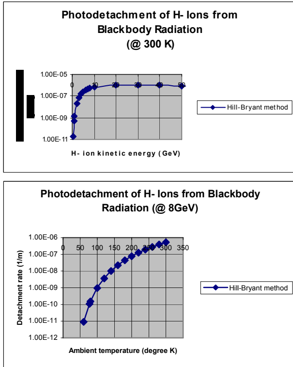
Figure 2: Top – energy dependence of blackbody radiation stripping; bottom – temperature dependence.
