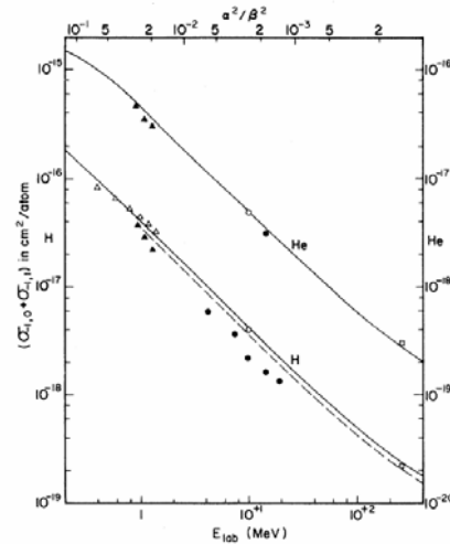
Figure 4: Energy dependence of electron loss cross section for H^- incident on H and He atoms [8].
