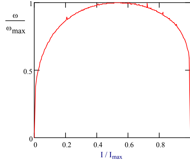
Dependence of synchrotron frequency on the action
