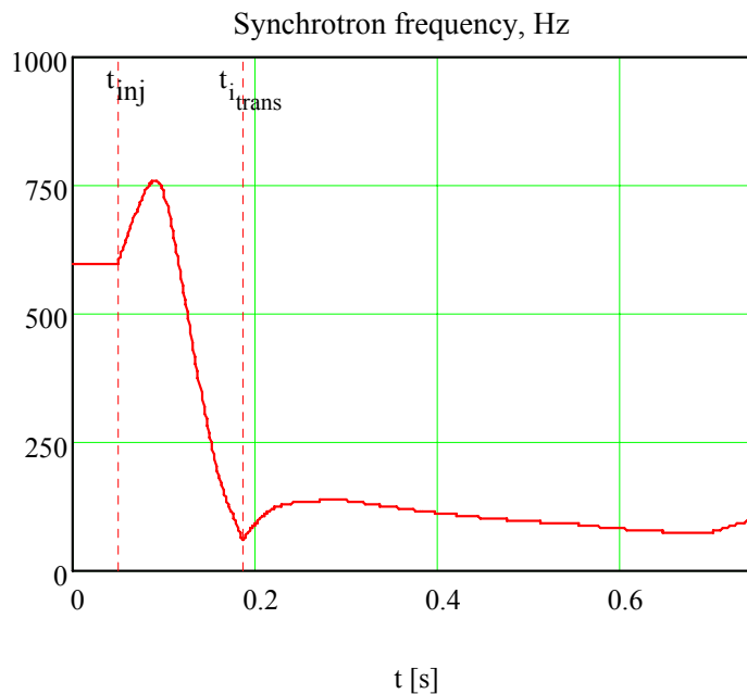
Figure 3. Dependence of RF power, maximum synchrotron frequency and incoherent tune shifts on the accelerating time.
