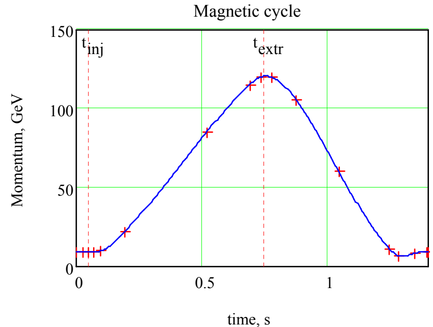
Dependence of beam momentum on time during MI magnetic cycle
